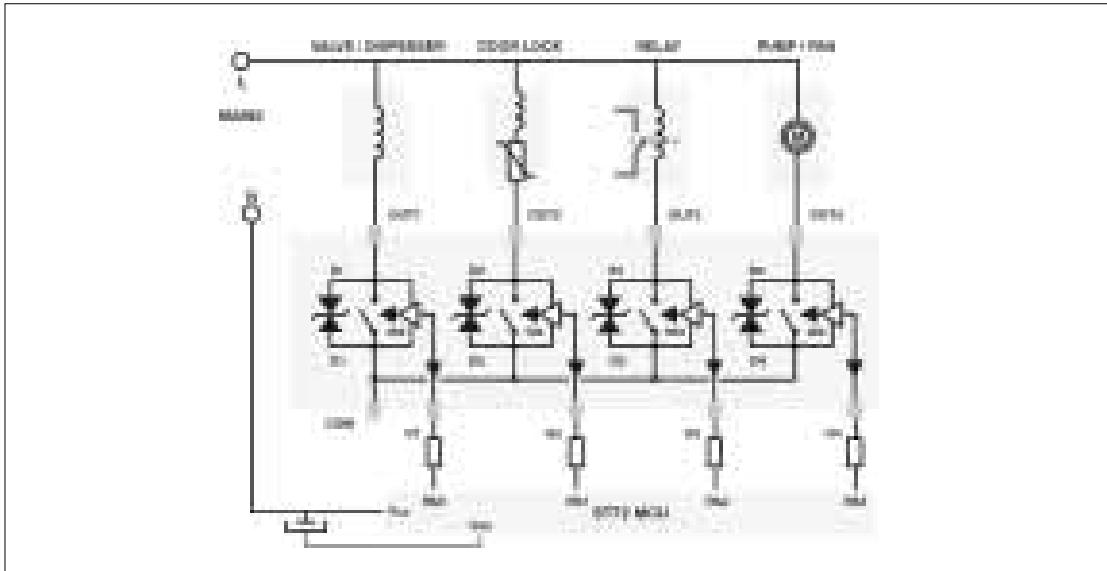
Typical configuration in washing machine
