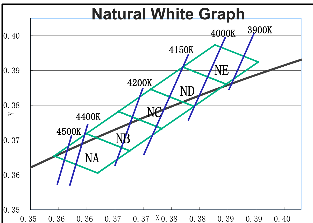
ANSI Natural White Color bin structures
