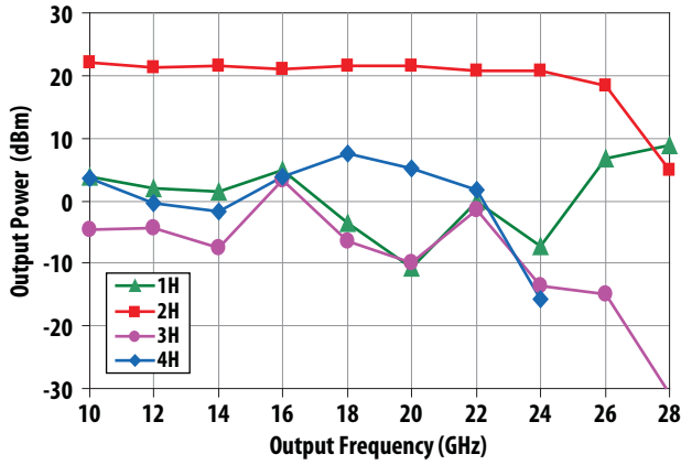
Figure 1. Output Power vs. Output Frequency @ \text{Pin} = 0\text{ dBm}
