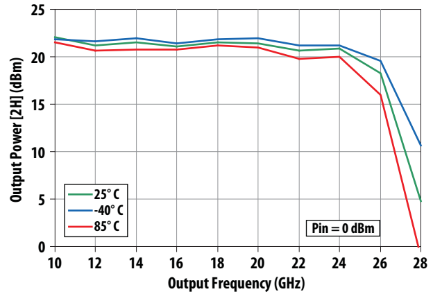
Figure 4. Output Power vs. Output Frequency @ \text{Pin} = 0\text{ dBm} over Temperature
