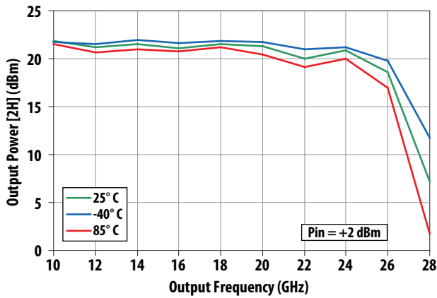
Figure 5. Output Power vs. Output Frequency @ \text{Pin} = +2\text{ dBm} over Temperature
