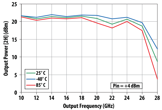
Figure 6. Output Power vs. Output Frequency @ \text{Pin} = +4\text{ dBm} over Temperature
