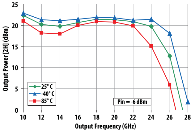
Figure 3. Output Power vs. Output Frequency @ \text{Pin} = -6\text{ dBm} over Temperature
