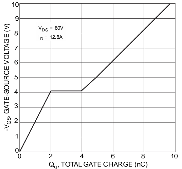
Figure 10 Gate-Charge Characteristics
