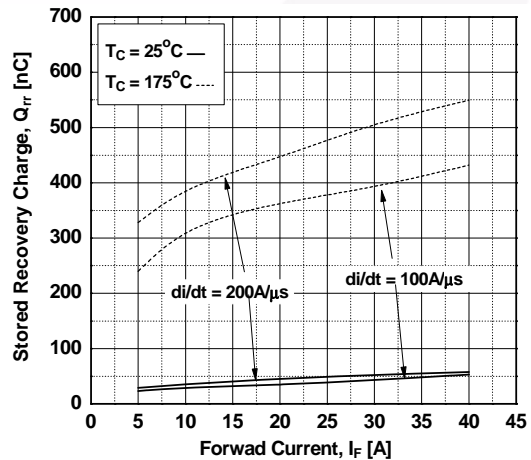
Figure 24. Stored Charge
