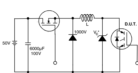
Fig. 19 - Clamped Inductive Load Test Circuit
