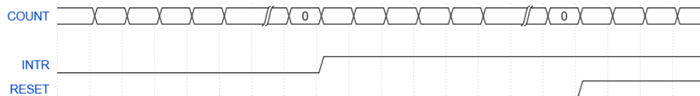
Figure 15. WDT Behaviour for Response Mode of 1
