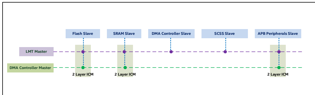
Figure 5 Multi-Layer AHB fabric with ICM
