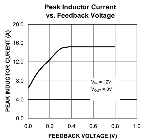
Figure 4. MIC27600 Current Limit Foldback Characteristic
