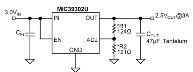
MIC39302 Adjustable Output Application (*See Minimum Load Current Section)
