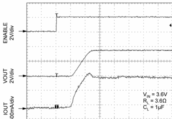
TIME 100µs/div
