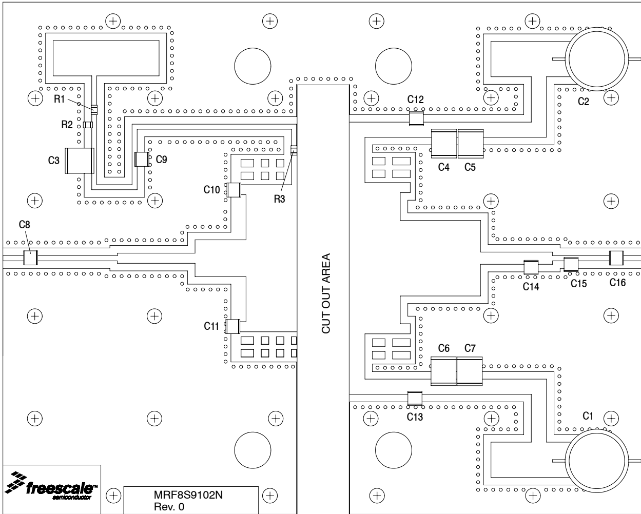
Figure 1. MRF8S9102NR3 Test Circuit Component Layout
