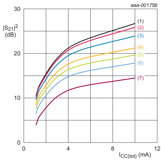
T_{amb} = 25\text{ }^{\circ}\text{C}; V_{CC} = 3\text{ V}; P_i = -30\text{ dBm}. (1) f = 150\text{ MHz} (2) f = 450\text{ MHz} (3) f = 900\text{ MHz} (4) f = 1500\text{ MHz} (5) f = 1900\text{ MHz} (6) f = 2400\text{ MHz} (7) f = 3500\text{ MHz}
