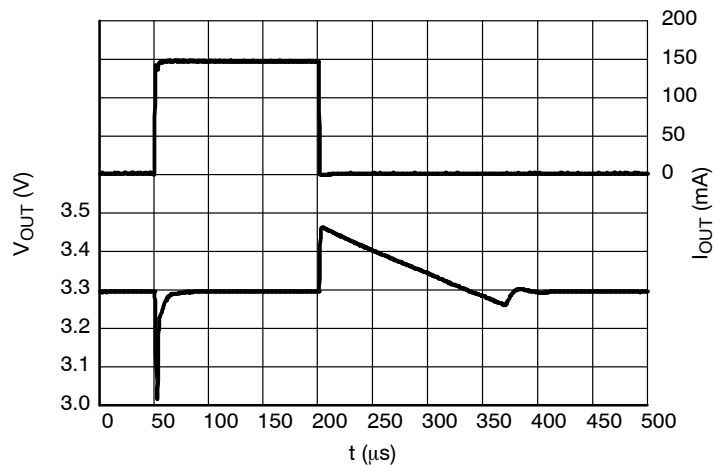
Figure 32. Load Transients, 3.3 V Version, I_{OUT} = 1 - 150 mA, t_R = t_F = 0.5 \mu s, V_{IN} = 3.8 V
