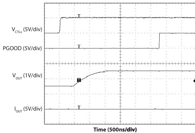
Start Up into Pre-Biased Output ( V_{OUT} = 1.5\text{V} )
