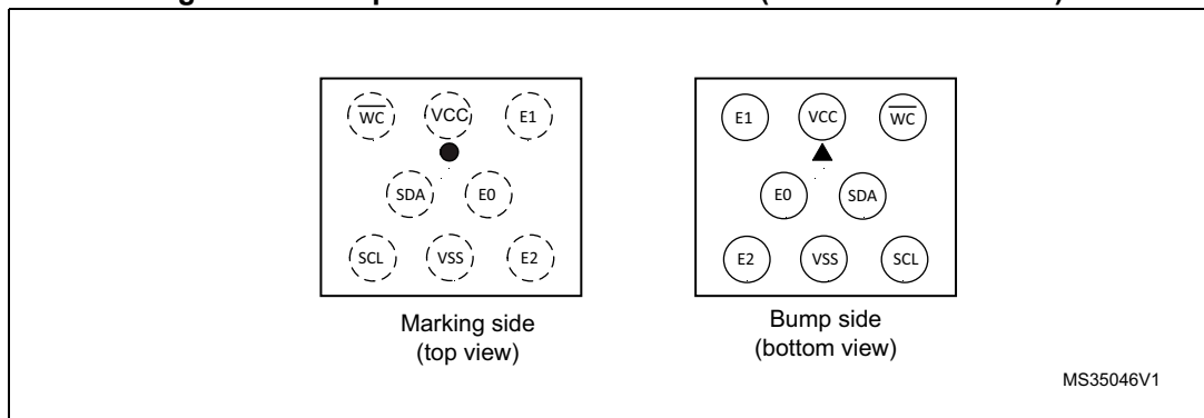
Figure 6. 8-bump thin WLCSP connections (M24C64-DFCT6TP/K)
