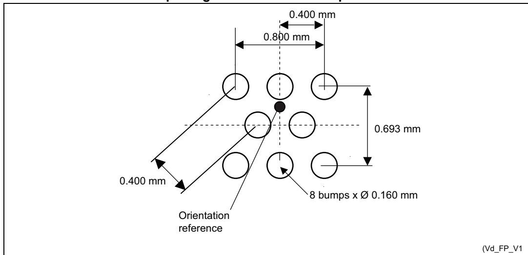
Figure 29. Thin WLCSP- 8-bump, 1.073 x 0.959 mm, wafer level chip scale package recommended footprint
